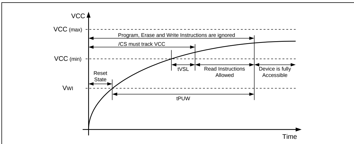
Figure 59a. Power-up Timing and Voltage Levels
